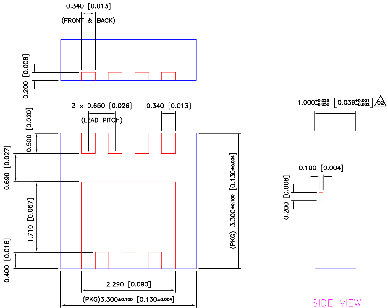
BOTTOM VIEW
